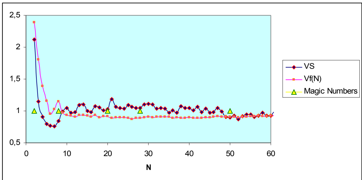
Figure 8: Fluctuations in the model parameters (28) over trend lines in the case of light nuclei.
