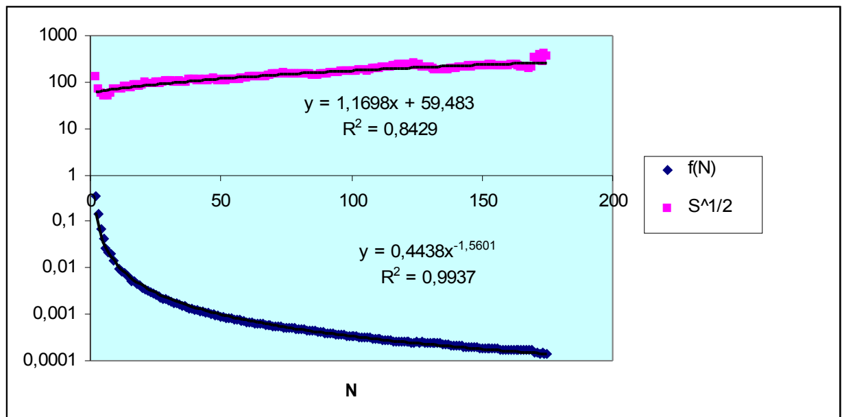
Figure 6: Interaction parameter f(N) = Sb_0(1 - u^2) and parameter S^{1/2} = \hbar k_p / m_e c characterizing the motion of matter in the fifth dimension as a function of number of neutrons at Sb_0 = 1 .
