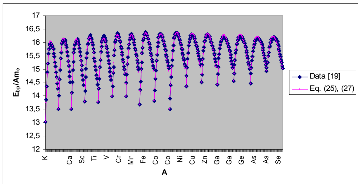
Figure 3: Binding energy per nucleon as a function of mass number calculated for a number of isotopes of chemical elements on the model (25), (27) and according to [19].
