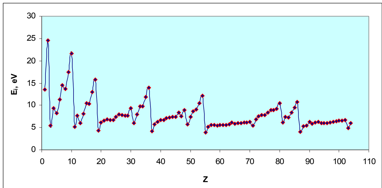
Fig. 1: The dependence of the ionization energy of the atomic number of the data [5].
