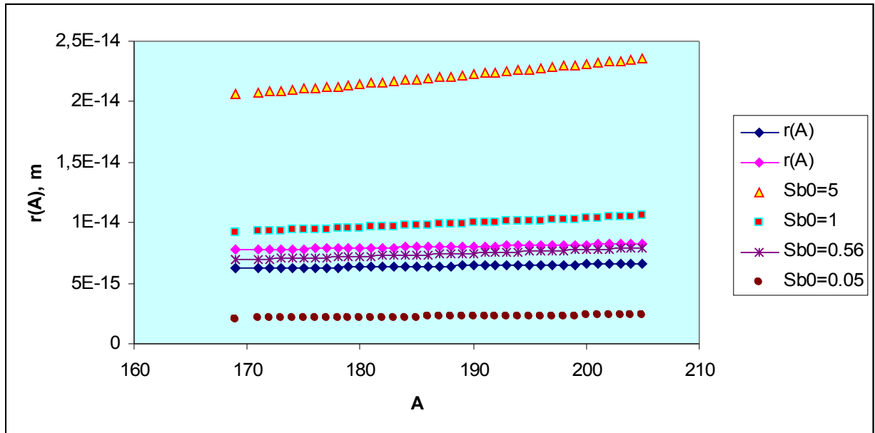
Figure 5: Gold nuclei isotope radius and the characteristic scale of the model as function of mass number.
