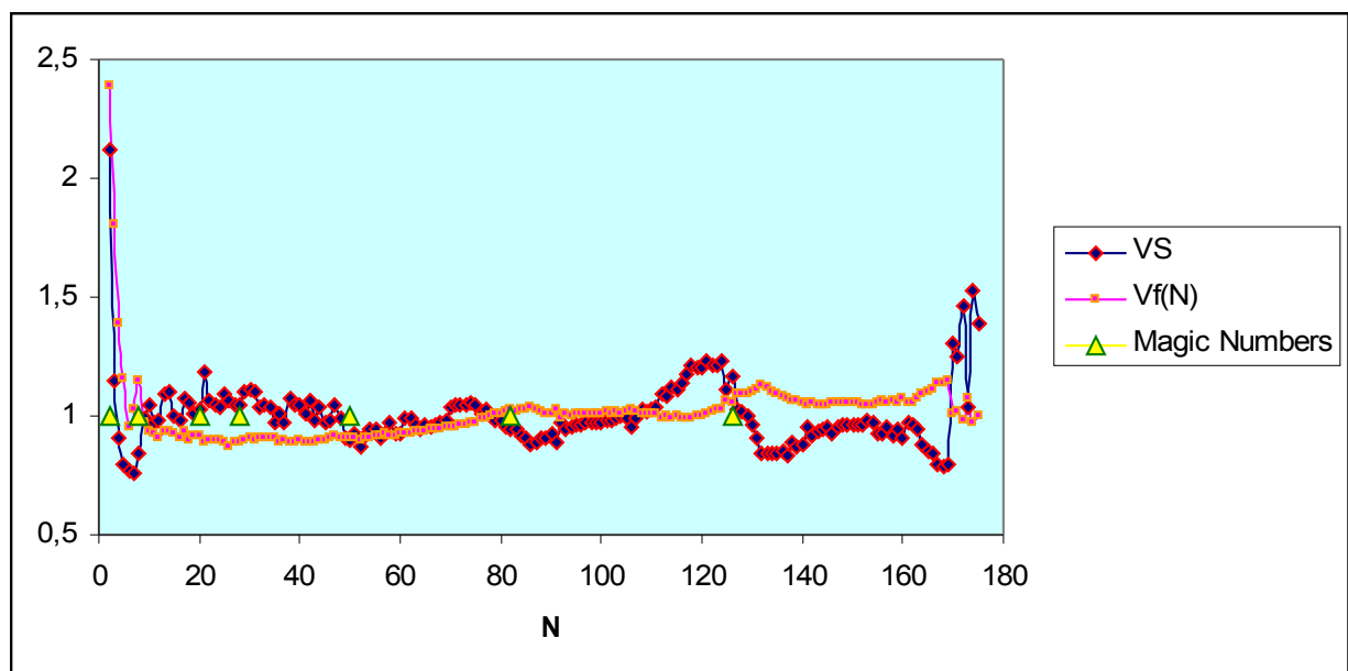
Figure 7: Fluctuations in the model parameters (28) over trend lines:
